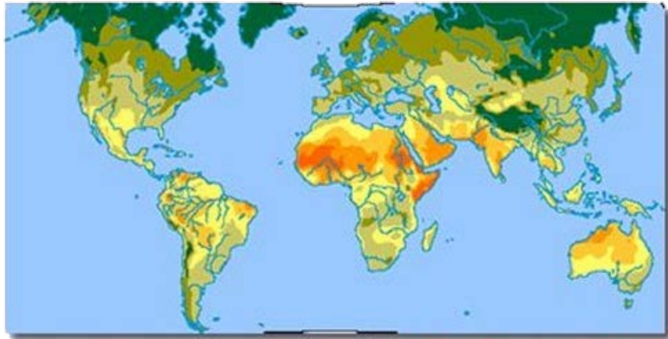
Mean Annual Potential Evapotranspiration. Source: UNEP World Atlas of Desertification
